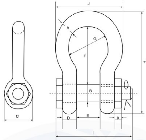
Safety Pin Bow Shackles Grade S
